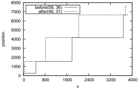
Pima Diabetes (2, 12%)
