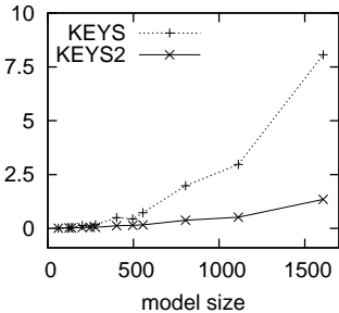
runtimes (secs)
