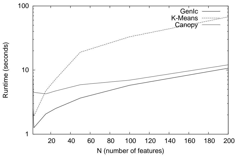
ap214 - Clustering - Number of Dimensions vs Runtimes
