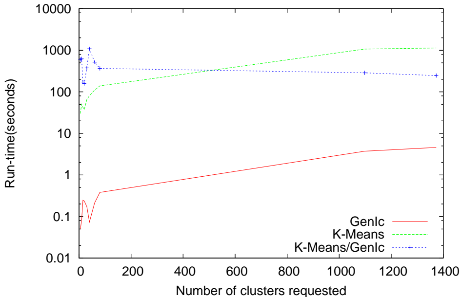
K-Means vs Genlc - STEP ap214 (n=1373)
