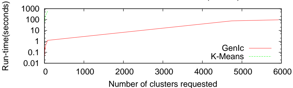
K-Means vs Genlc - Florida Law (n=5930)
