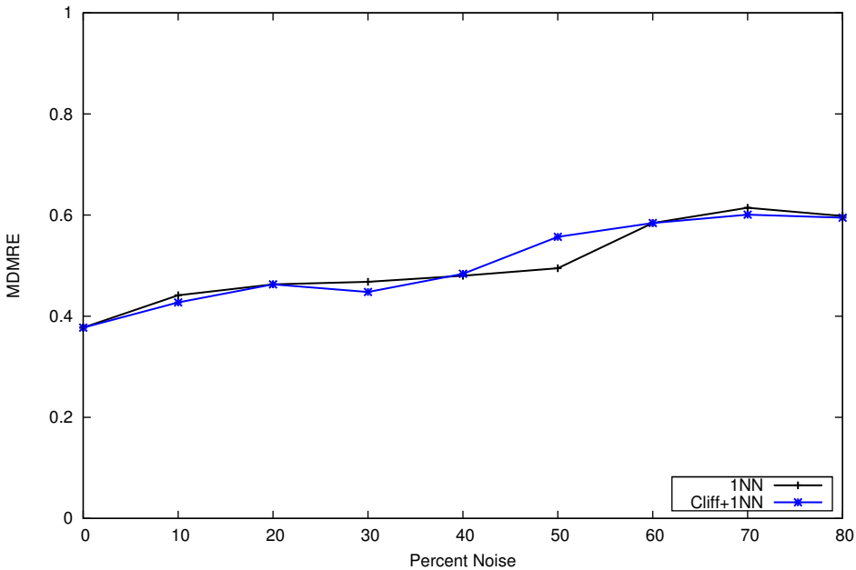
MDMRE for albrecht
