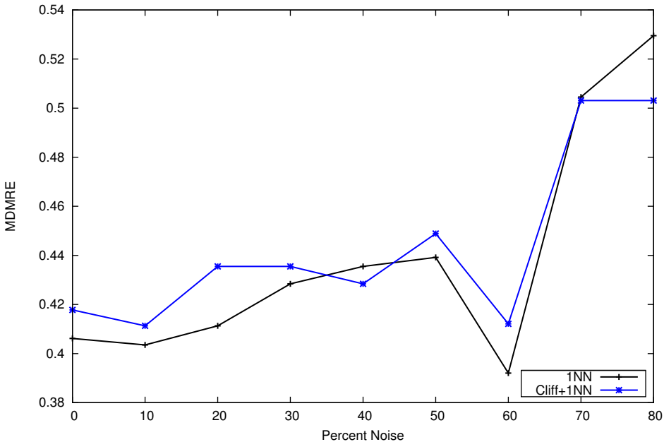
MDMRE for desharnais
