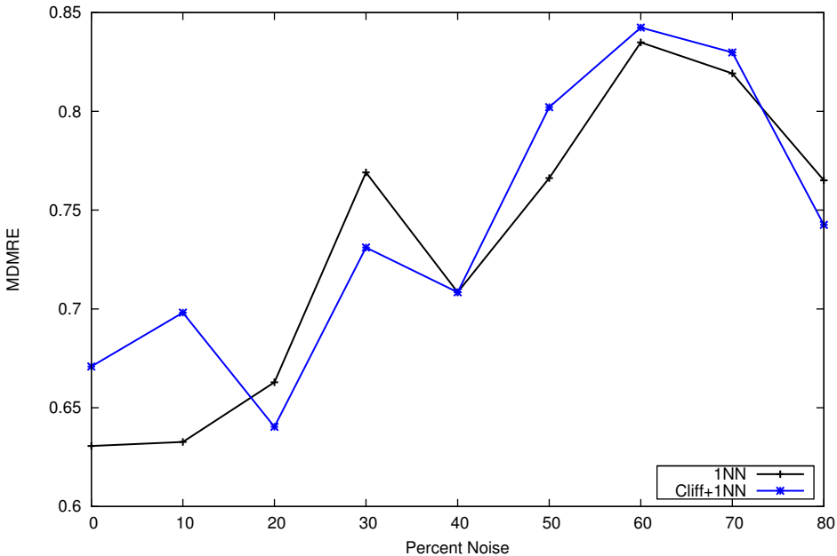
MDMRE for finnish
