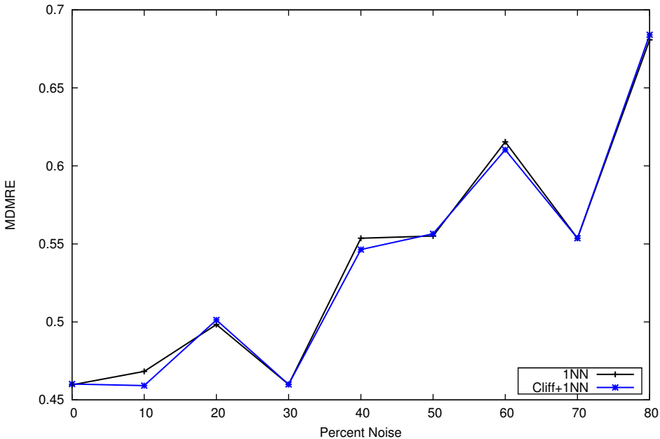
MDMRE for maxwell
