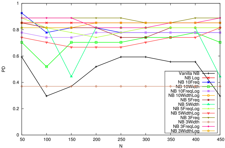
PD for True Class in KC2
