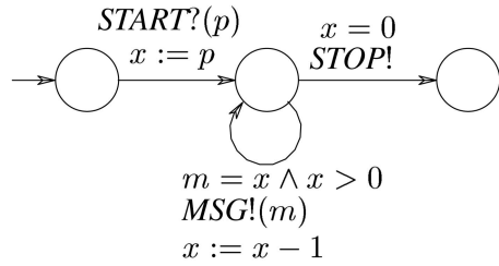
Fig. 1. Sample IOSTS S .
