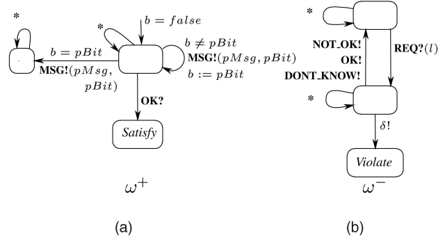
Fig. 7. Properties. (a) Possibility. (b) Safety.
