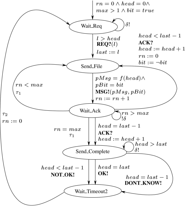
Fig. 8. Suspended BRP.
