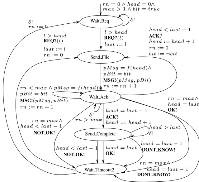
Fig. 9. Determinized BRP.
