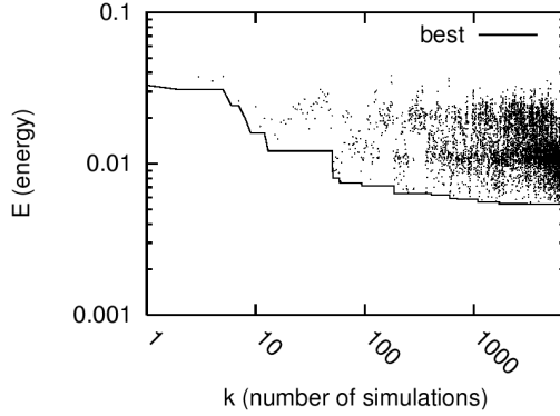
Figure 5: Processing a JPL requirements model.
