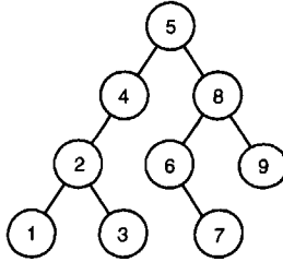
Figure 4.4: A binary search tree.
