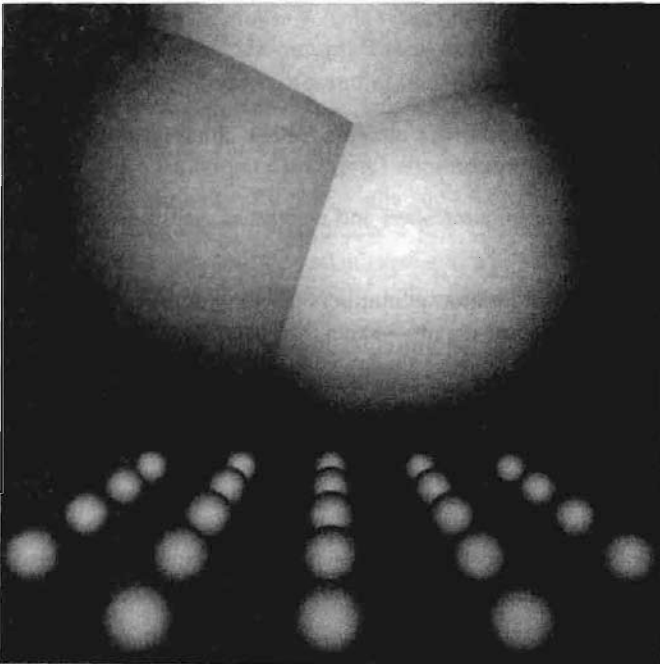
Figure 9.7: Ray-traced image.
