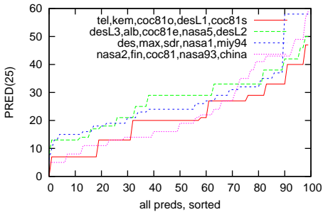
Performance, grouped by data sets
